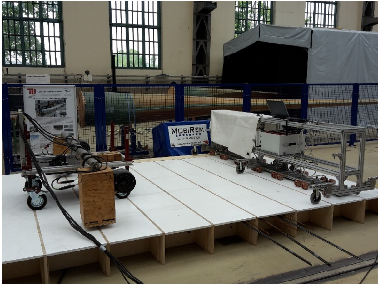
Figure 14: Test platform for re-adjusting individual reinforcement arrangements for prestressing steel as well as for slack steel, suitable for each of the three measuring units (REM 40, REM 150 and REM 350).
