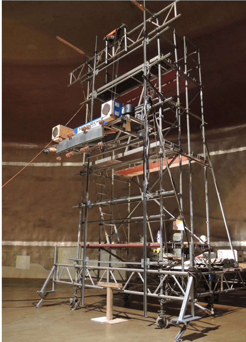
Figure 15: Examination of horizontally running tendons in the wall area of prestressed tank containers using a lifting platform.
