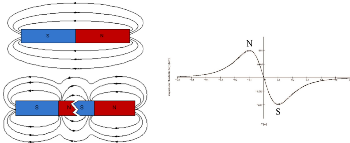
Figure 2: At the breaking point there is a magnetic north pole (N) and a magnetic south pole (S) opposite each other (picture on the left). The measurement signal (picture on the right) shows a characteristic course. Between the two poles (extreme values) is the turning point of the signal curve of the transverse component, which shows the exact center of the break point.
