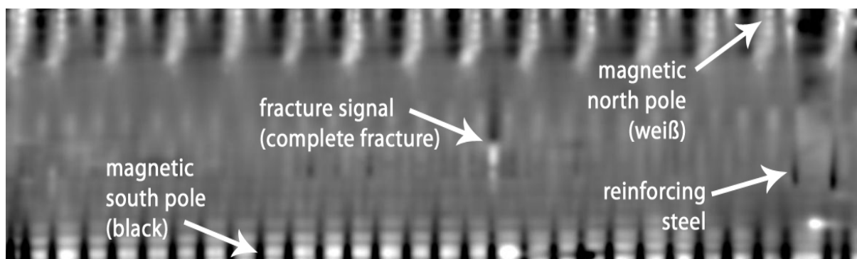
Figure 19: Evaluated magnetic image of a measuring track with the RM 350 with identification of the tendons and a fractured signal.
